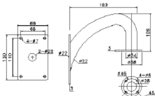
FSD-230WB
