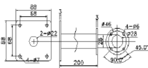
FSD-230CB
